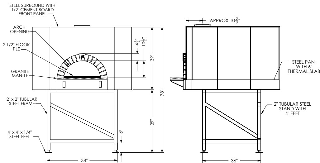
FRONT VIEW
