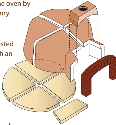
OVEN COMPONENTS
