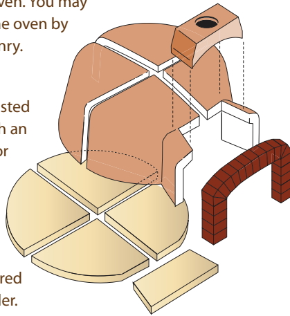
OVEN COMPONENTS
