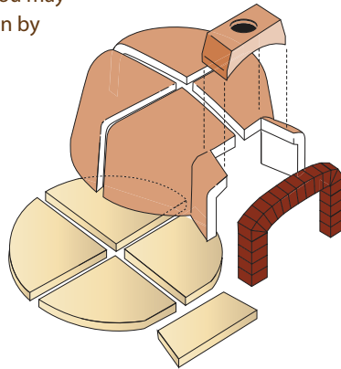
OVEN COMPONENTS
