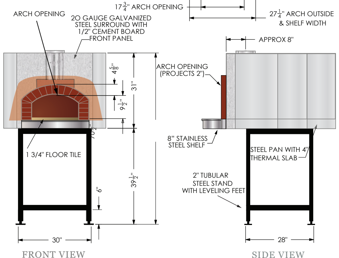
OVEN COMPONENTS
