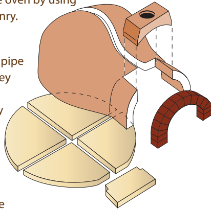
OVEN COMPONENTS
