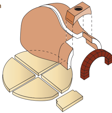
OVEN COMPONENTS
