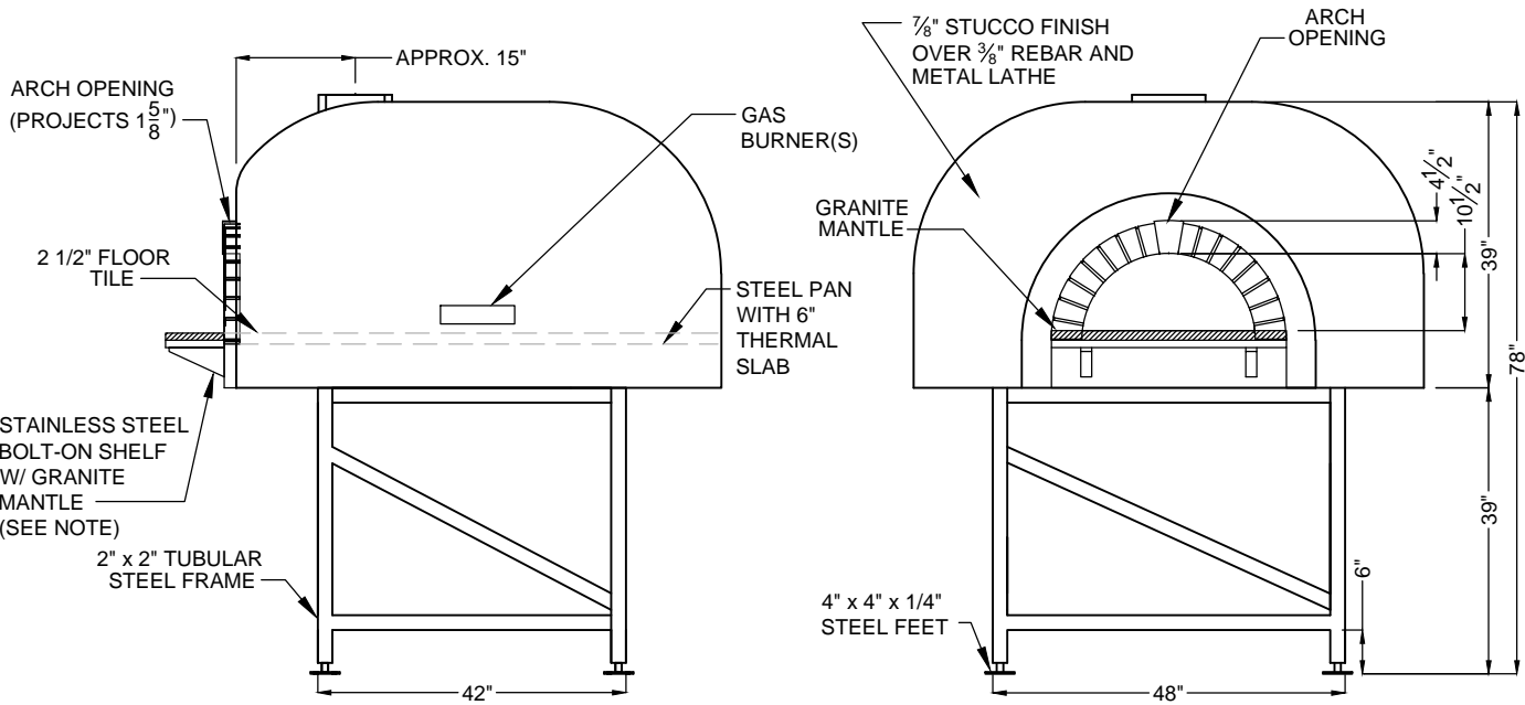
SIDE VIEW
